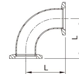
90° Elbow Flange
