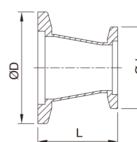
Conical Reducer
