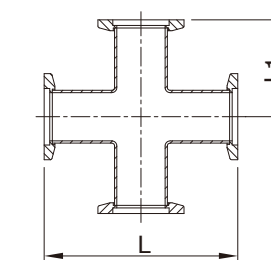
4-Way Cross Flange
