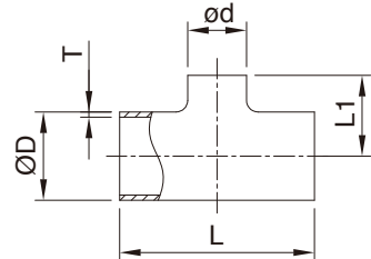
Reducing Tee
