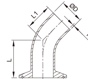
L2KM WELD/CLAMP 45° ELBOW
